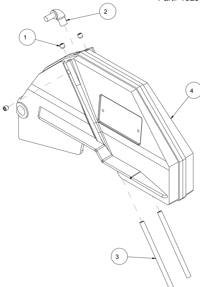
Blade Guard Part# 152582
